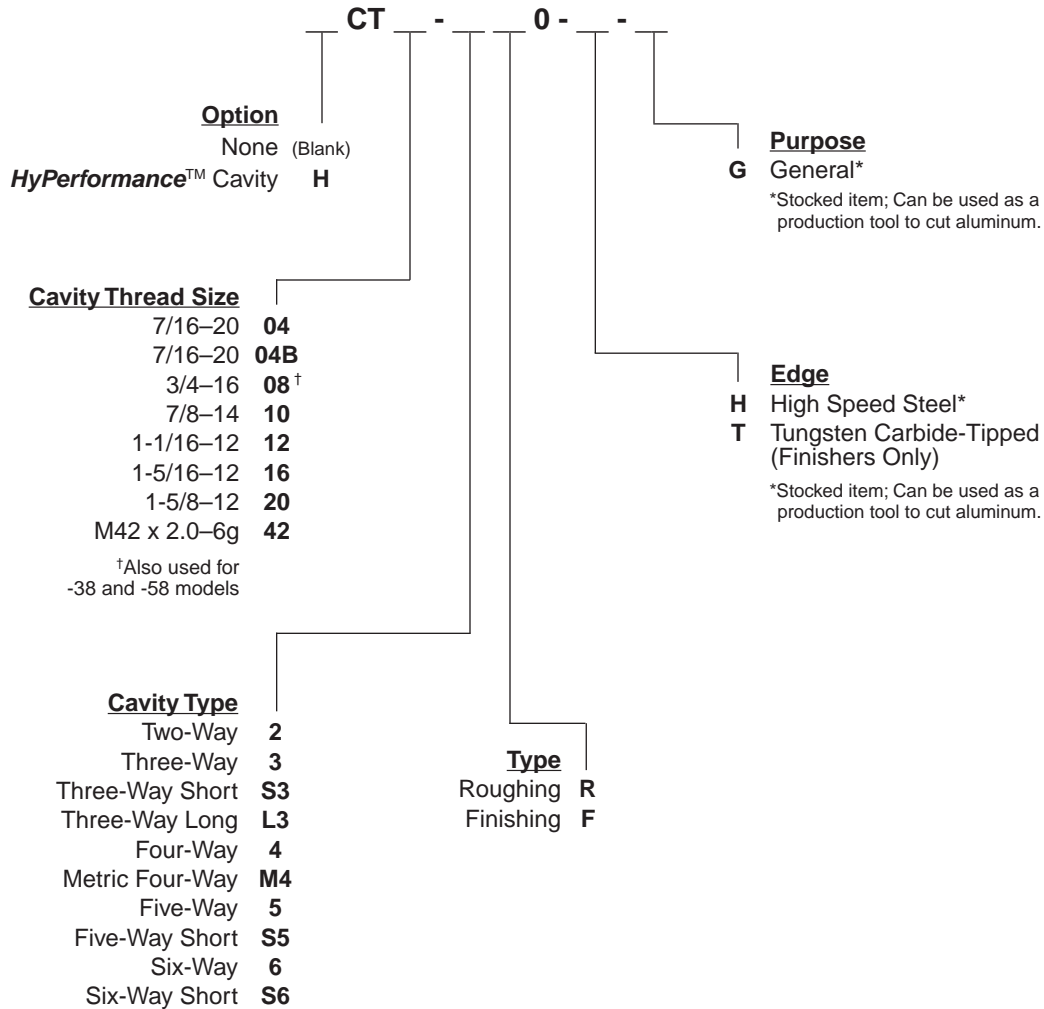
Cavity Rougher
