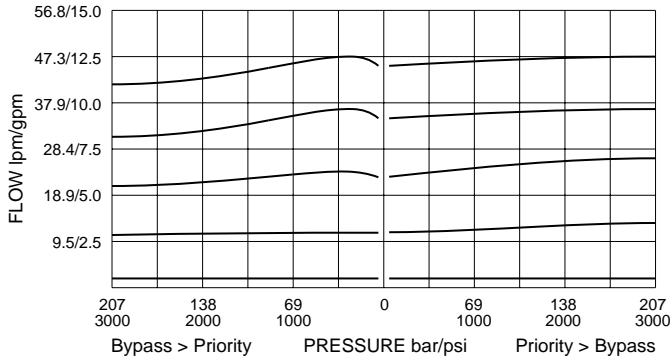
Priority Flow vs. Load Pressure at 75.7 lpm/20.0 gpm Inlet Flow 32 cSt/150 ssu oil at 40°C
