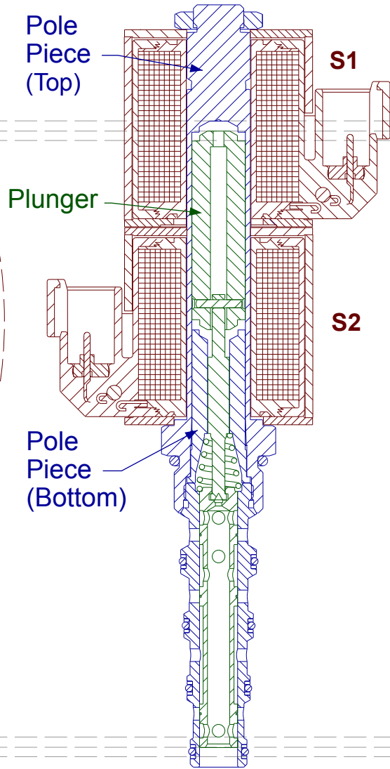
Fig. 2 Neutral De-Energized Valve Spool Centered
