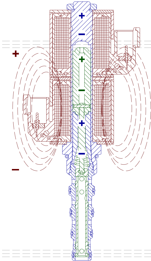
Fig. 1 Coil 2 Energized Valve Spool Shifted Down
