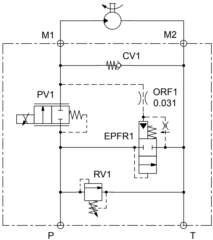
Proportional Motor Control Circuit with orifice dampening the load signal to an EPFR valve.
