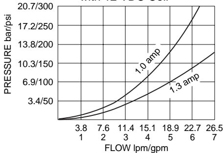
TYPICAL PRESSURE DROP ② to ① with 12 VDC Coil
