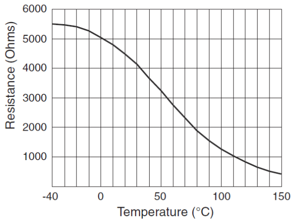
TEMPERATURE vs. RESISTANCE CHARACTERISTICS
