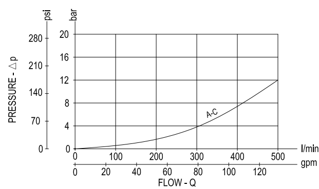
\Delta p = f(Q) Pressure drop - Flow rate characteristic Lifting (A->C)
