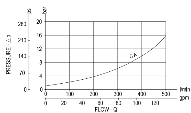
\Delta p = f(Q) Pressure drop - Flow rate characteristic Lowering (C->A), main stage (3) completely open.
