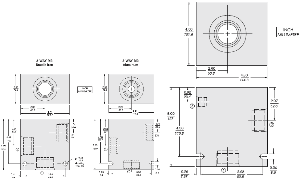
3-WAY S3 and S3A Ductile Iron, H-Series
