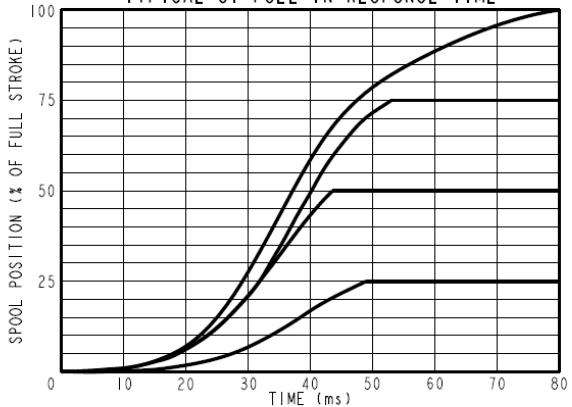
TYPICAL S1 PULL-IN RESPONSE TIME
