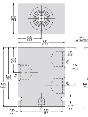
4-WAY M4 PD-Type Aluminum or Ductile Iron
