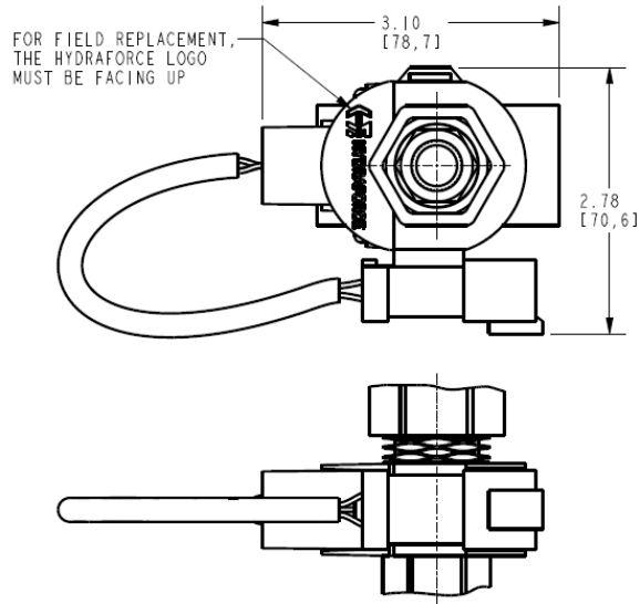
N3 - DUAL OUTPUT (DT04-4P)
